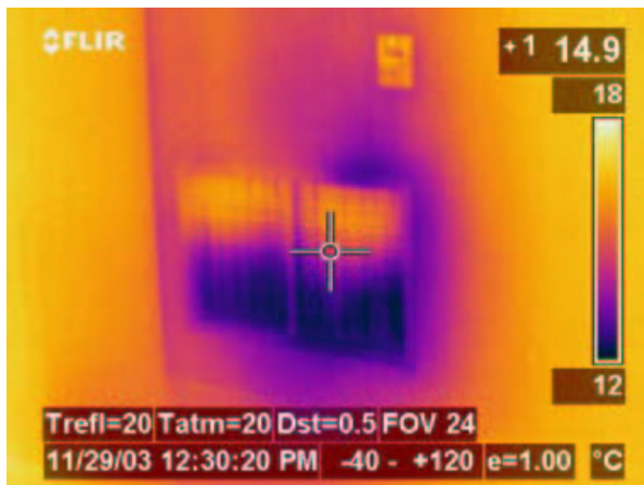
Figure 9. Thermogram/photo showing non-uniform air distribution pattern from supply register
