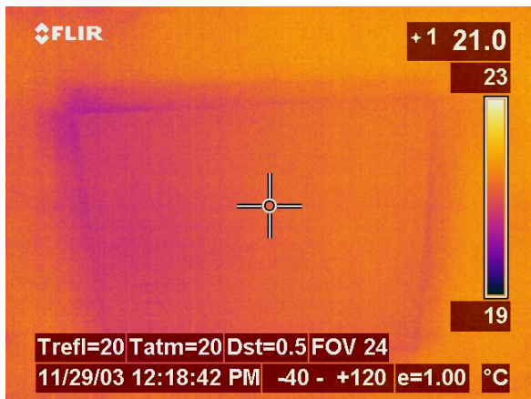
Figure 8. Thermogram/photo showing non-uniform air distribution pattern from supply register
