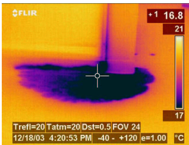
Figure 1. Thermogram/photo showing water intrusion from plumbing leak inside wall behind fountain
